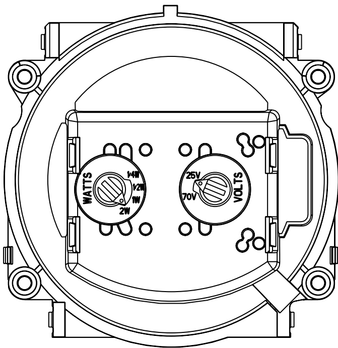
FIGURE 3. SPEAKER WATTAGE AND VOLTAGE SETTINGS:
