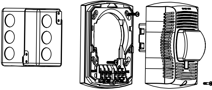
FIGURE 4: WALL MOUNT PRODUCT WITH TRIM RING:
