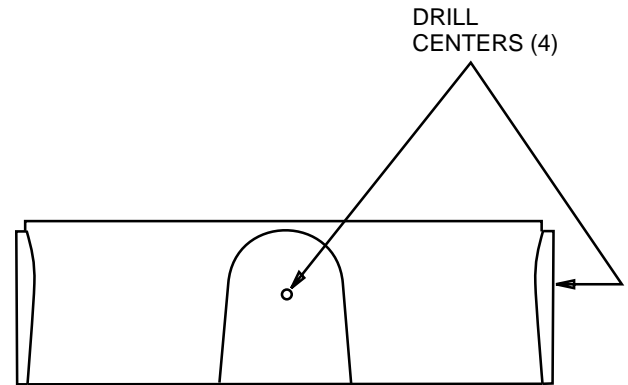
Figure 1. Drill centers:
