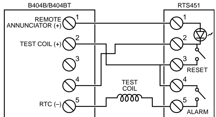
Figure 3. RTC Wiring Diagram:
