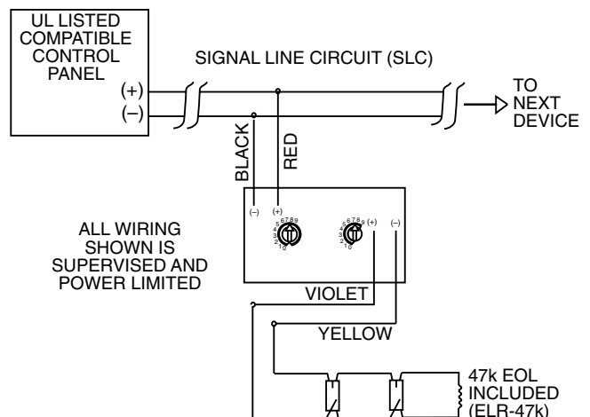
Figure 2. Typical 2-wire style B initiating circuit configuration:
