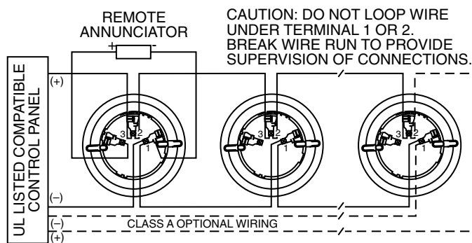
FIGURE 1. WIRING DIAGRAM:
